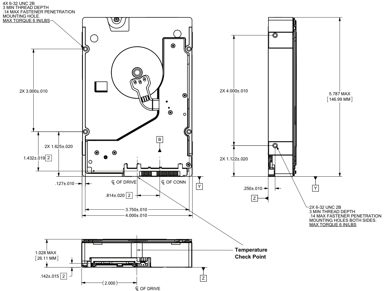
Figure 3 Mounting dimensions
